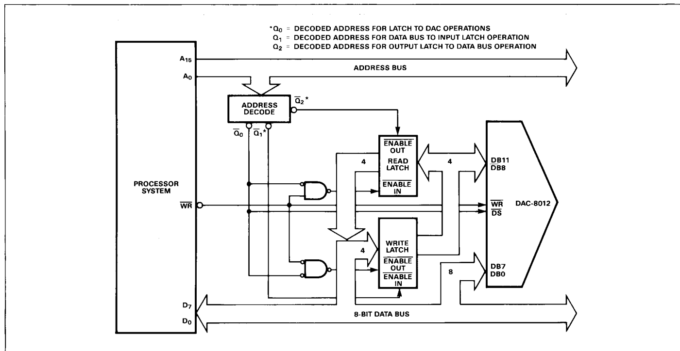
FIGURE 7: 8-Bit Processor to DAC-8012 Interface
