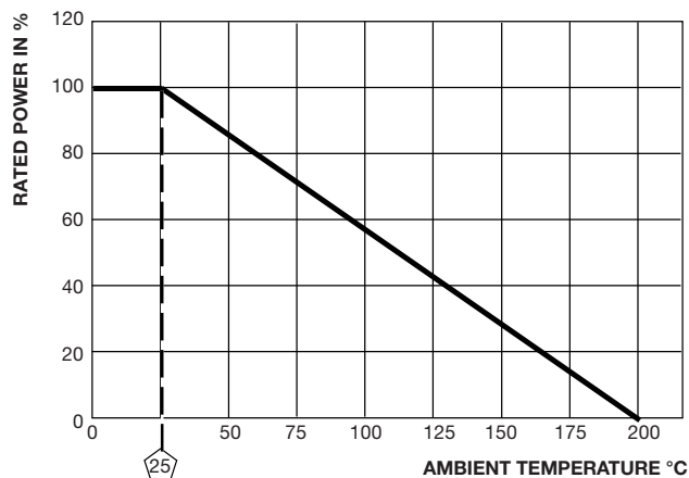
Derating
