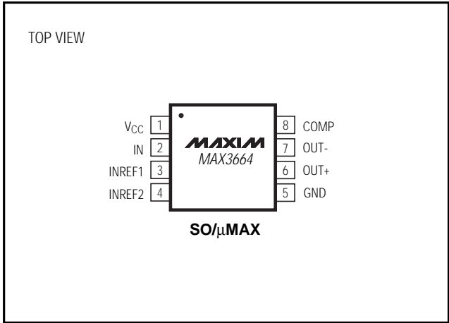
Pin Configuration
