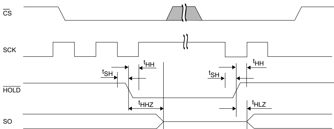
Figure 36. \overline{HOLD} Timing
