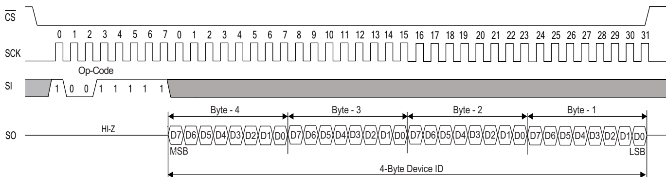
Figure 27. RDID Instruction
