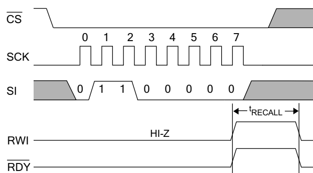
Figure 39. Software RECALL Cycle
