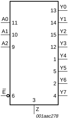
Fig 3. Logic symbol
