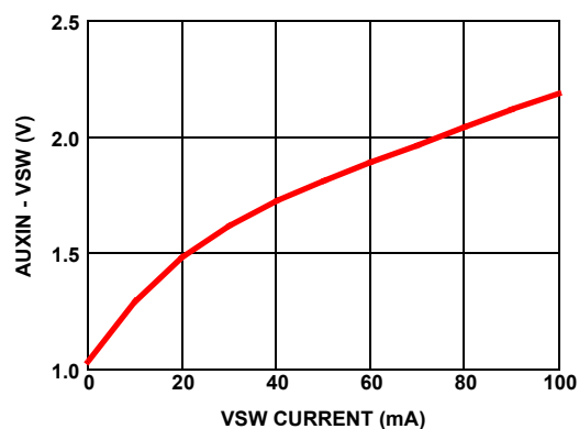
FIGURE 2. AUXIN - VSW vs I_{VSW} @ VPWR = 17V, +25°C
