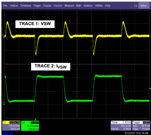
FIGURE 6. VSW TRANSIENT RESPONSE, 10mA TO 100mA STEP, VPWR = 18V, AUXIN = 15V, VSW = 12V Figure 6 depicts the transient response of VSW during a 10mA to 100mA step load when AUXIN is set to 15V and VPWR is set to 18V.
