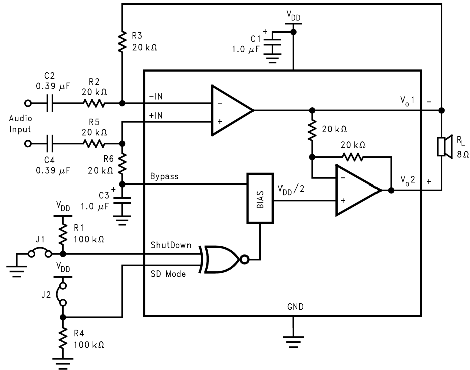
Figure 42. DIFFERENTIAL AMPLIFIER CONFIGURATION FOR LM4990
