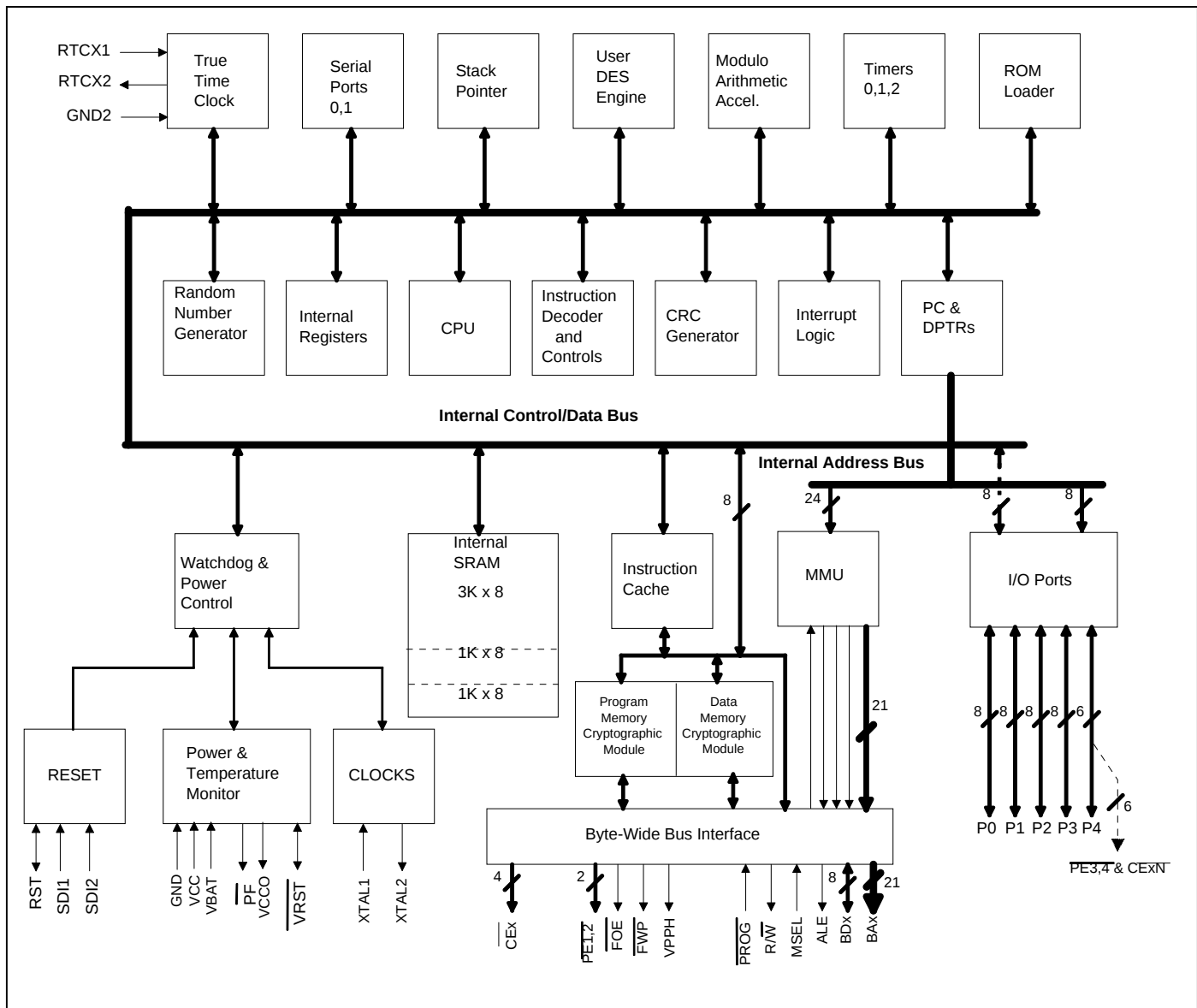
Figure 1. Block Diagram
