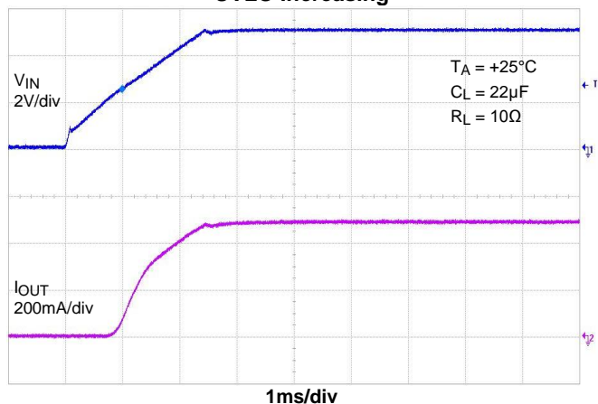
UVLO Increasing
