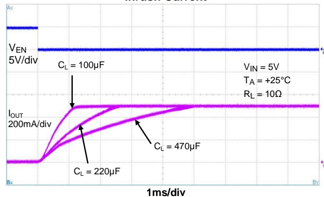
Inrush Current
