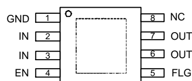
MSOP-8EP
