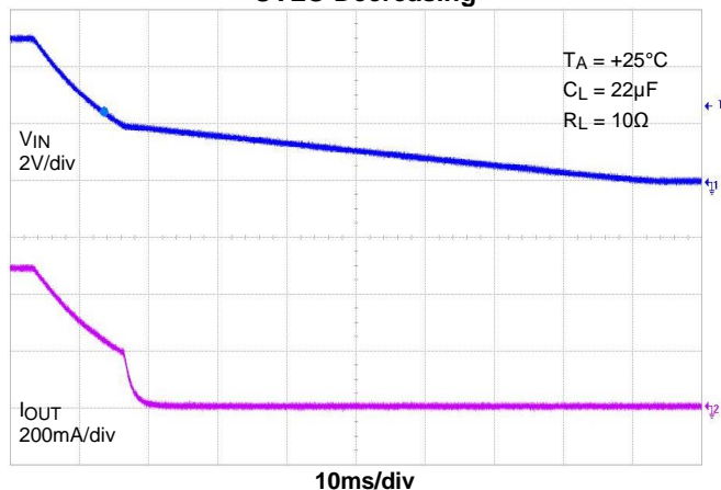
UVLO Decreasing
