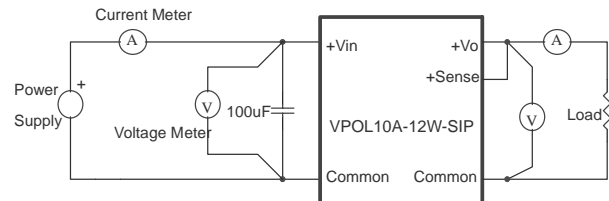
Figure 13. VPOL10A-12W-SIP Series Test Setup
