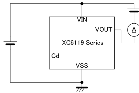
Circuit 6
