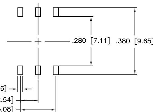
SUGGESTED LAND PATTERN
