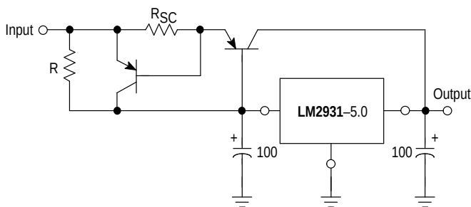
Figure 20. Current Boost Regulator with Short Circuit Projection
