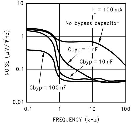
Figure 10. Noise Density
