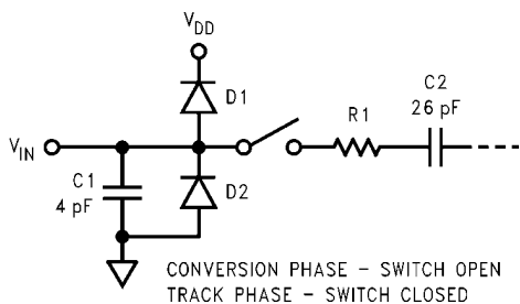
FIGURE 9. Equivalent Input Circuit
