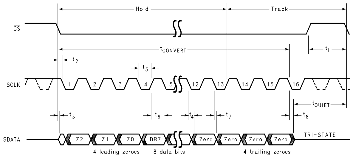
FIGURE 3. ADCS7478 Serial Interface Timing Diagram
