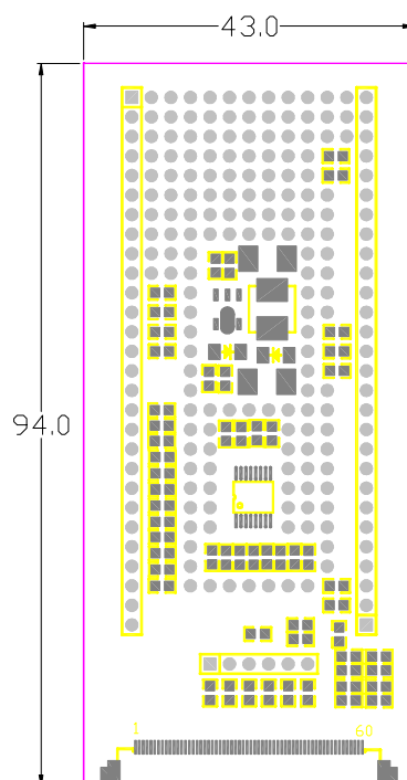
Figure 2. Outline Dimensions
