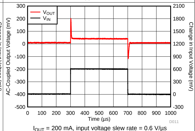
Figure 18. V_{IN} Transient
