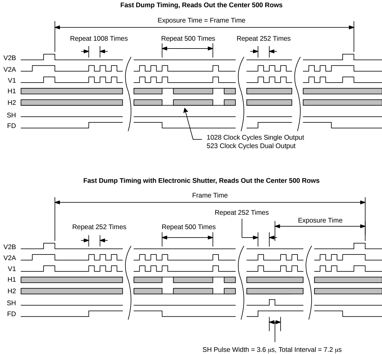
Figure 31. Fast Line Dump Timing Example
