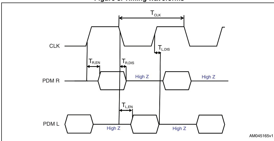
Figure 5. Timing waveforms
