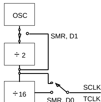
Figure 36. SCLK Circuit
