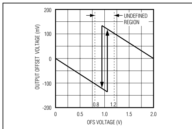
Figure 6. Offset Voltage
