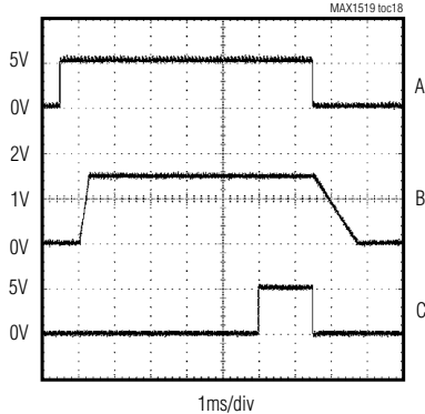
A. \overline{SHDN} , 5V/div B. 1.5V OUTPUT, 1V/div C. VROK, 5V/div R TIME = 64.9k \Omega
