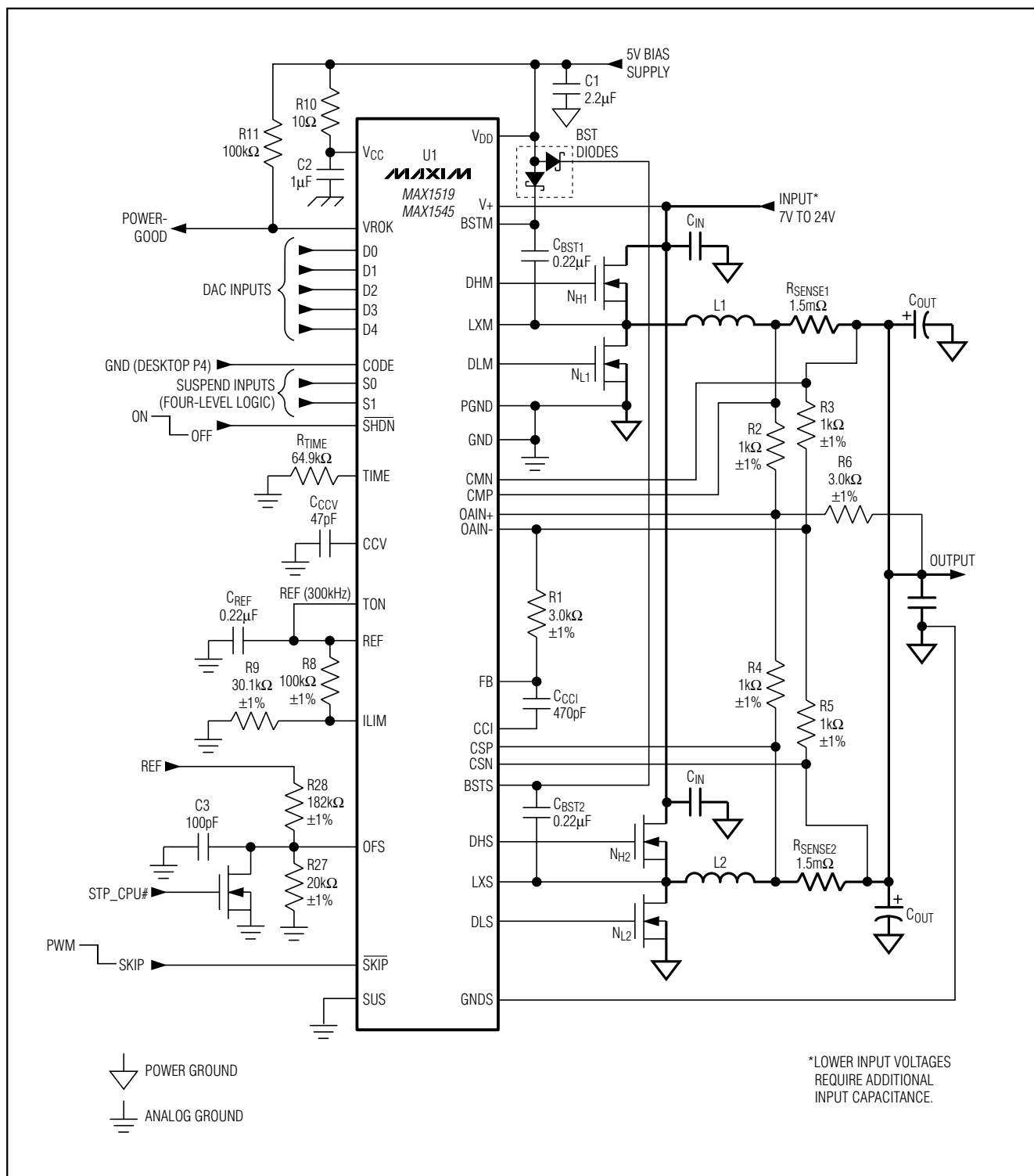
Figure 12a. Standard 4-Phase Desktop P4 Application Circuit (1st and 2nd Phases—MAX1519/MAX1545 Master)
