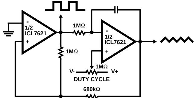
WAVEFORM GENERATOR
