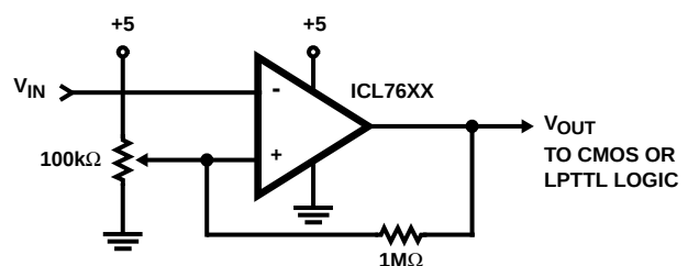
FIGURE 2. LEVEL DETECTOR
