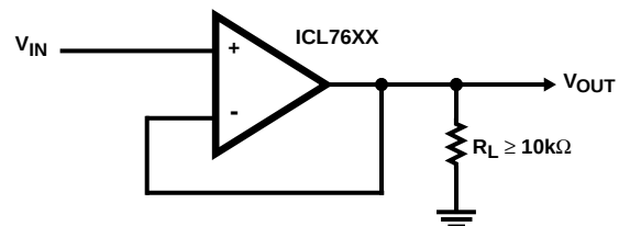
FIGURE 1. SIMPLE FOLLOWER
