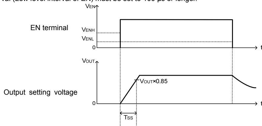
Figure 35. Timing Chart with Enable Control
