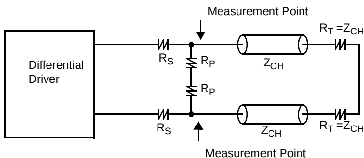
Figure 2. Equivalent Circuit
