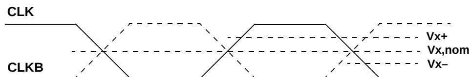
Figure 6. Crossing-point Voltage
