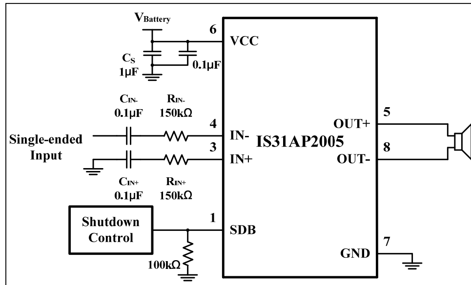
Figure 2 Typical Application Schematic with Single-ended Input
