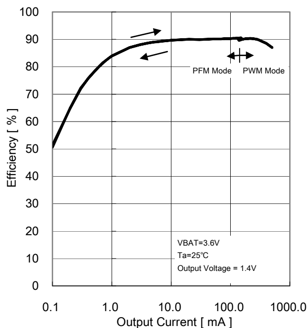
Figure 23. Efficiency vs Output Current (SWRE4 Efficiency)
