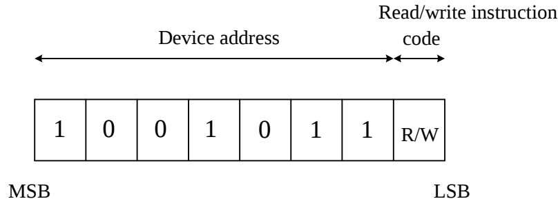
Figure 13. Device Addressing (Device address is "1001011" or "1001100".)
