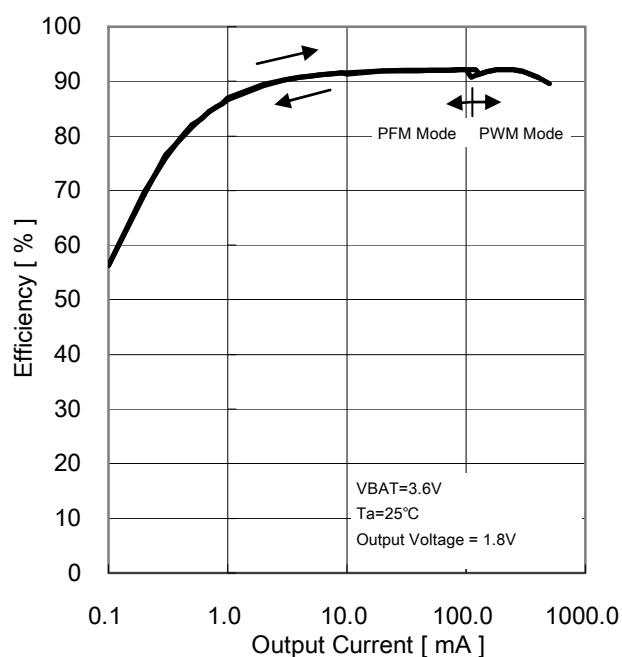
Figure 21. Efficiency vs Output Current (SWREG2 Efficiency)
