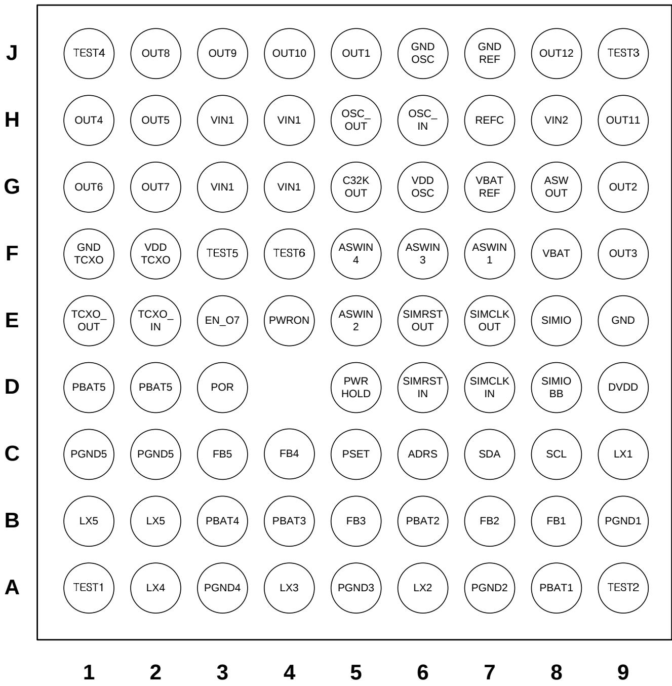
Bottom View Figure 2. Pin Configuration
