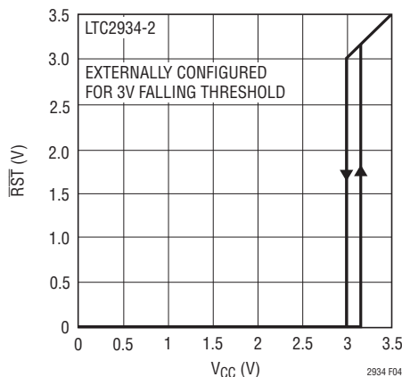
Figure 4. \overline{RST} vs V_{CC}
