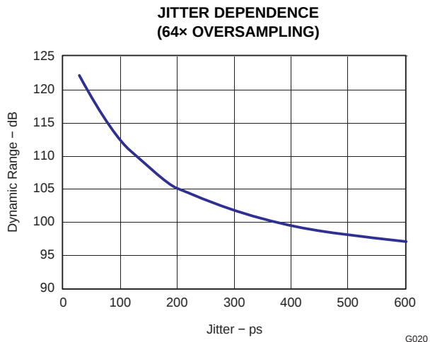
Figure 38. Jitter Sensitivity
