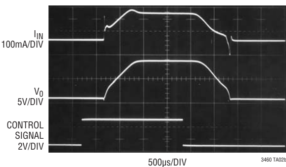
Input Current and Output Voltage
