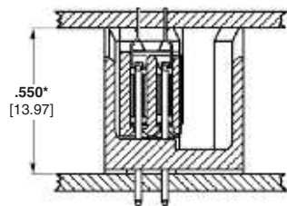
Figure 4 Double-Row, Two-Piece Receptacle and Two-Piece Shrouded Header *Mod II Shrouded Header Height is .440 [11.18] for a total stack height of .898 [22.80]
