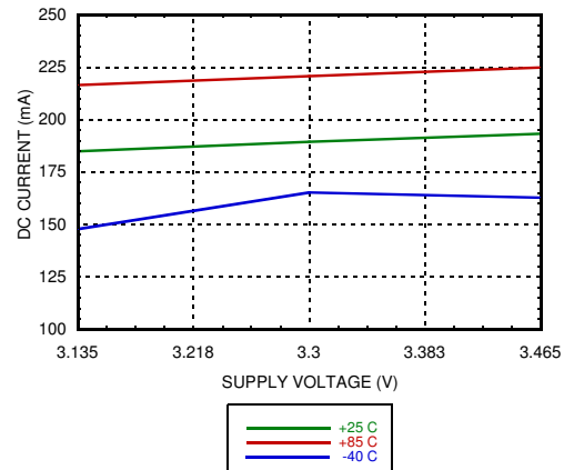
DC Current vs. Temperature [2][5]
