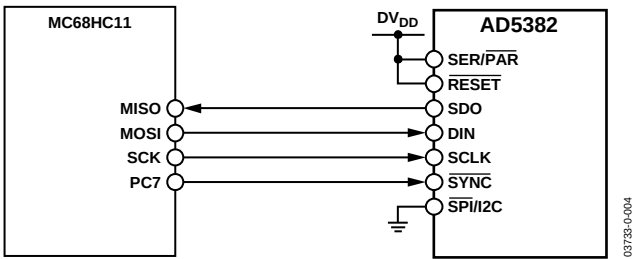
Figure 34. AD5382-to-MC68HC11 Interface
