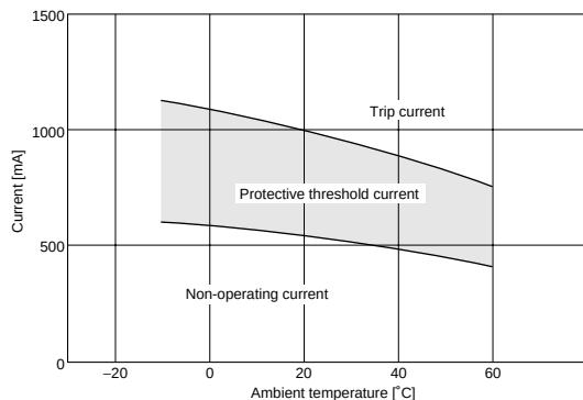
PTGL09AR1R8H2B51B0
