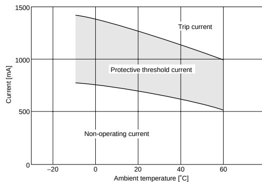
PTGL12AR1R2H2B51B0
