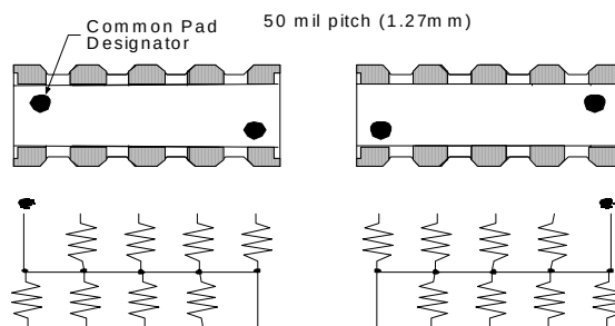
745X101 8 Resistors
