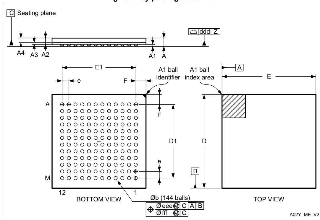
Figure 53. UFBGA - 144-pin, 10 x 10 mm, 0.80 mm pitch, ultra fine pitch ball grid array package outline
