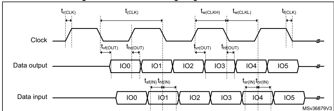
Figure 33. Quad SPI timing diagram - DDR mode
