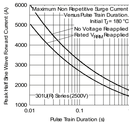
Fig. 11 - Maximum Non-Repetitive Surge Current
