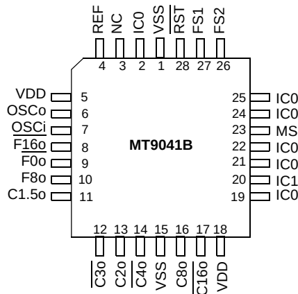
Figure 2 - Pin Connections
