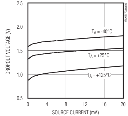
MINIMUM INPUT-OUTPUT DIFFERENTIAL vs. SOURCE CURRENT ( V_{OUT} = 10V )
