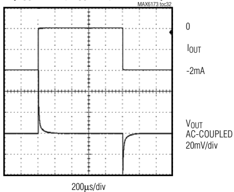
LOAD TRANSIENT ( V_{OUT} = 10V , C_{OUT} = 0 , 0 TO -2mA )
