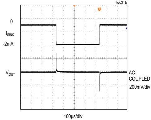
LOAD TRANSIENT ( V_{OUT} = 4.096V , C_{OUT} = 0 , I_{SINK} = 0 TO -2mA )
