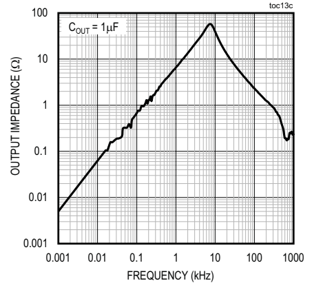
OUTPUT IMPEDANCE vs. FREQUENCY ( V_{OUT} = 4.096V )
