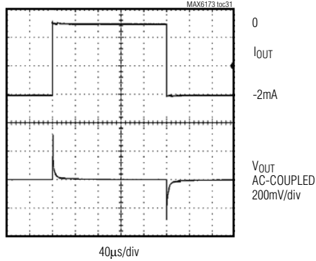
LOAD TRANSIENT ( V_{OUT} = 2.5V , C_{OUT} = 0 , 0 TO -2mA )
