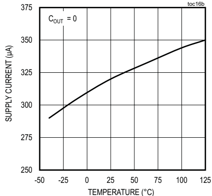
SUPPLY CURRENT vs. TEMPERATURE ( V_{OUT} = 4.096V )
