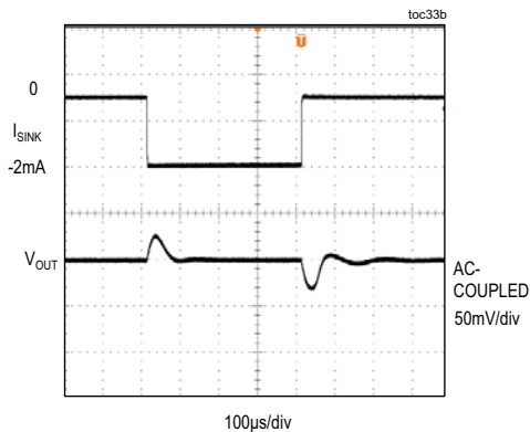
LOAD TRANSIENT ( V_{OUT} = 4.096V , C_{OUT} = 1\mu F , I_{SINK} = 0 TO -2mA )
