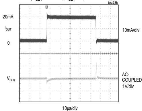
LOAD TRANSIENT ( V_{OUT} = 4.096V , C_{OUT} = 0 , 0 TO 20mA)
