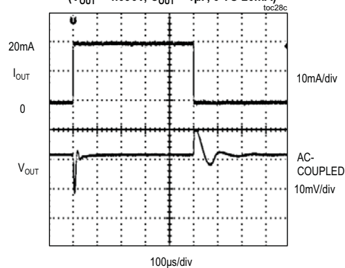
LOAD TRANSIENT ( V_{OUT} = 4.096V , C_{OUT} = 1\mu F , 0 TO 20mA)
