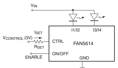
Two Diode Control with ON/OFF
