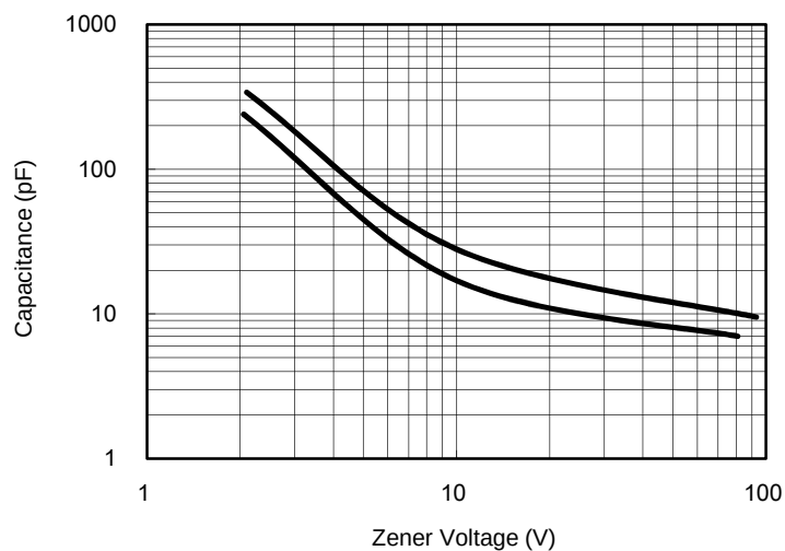
Fig. 5 Typical Capacitance
