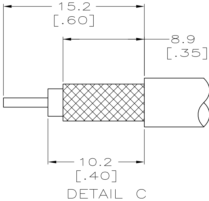
RECOMMENDED STRIP LENGTHS
