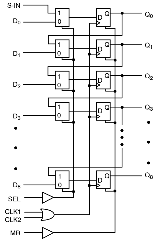
Figure 2. Logic Diagram
