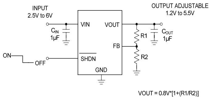
Figure 3 – LX8213-00 Adjustable Output Application Schematic
