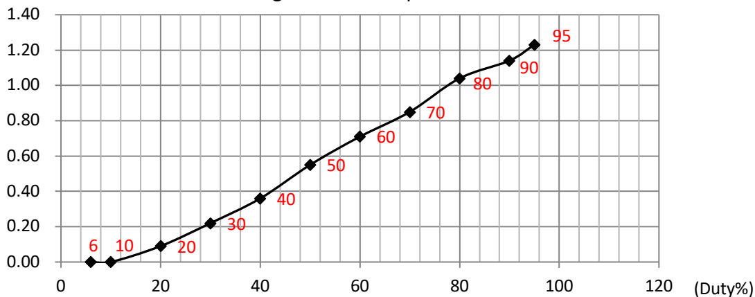
(A) Dimming-PWM VS Output Current
