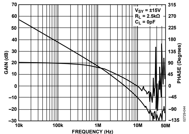
Figure 48. Frequency Response of Competitor A
