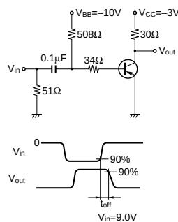
t_{stg} Test Circuit
