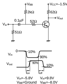
t_{on} , t_{off} Test Circuit
