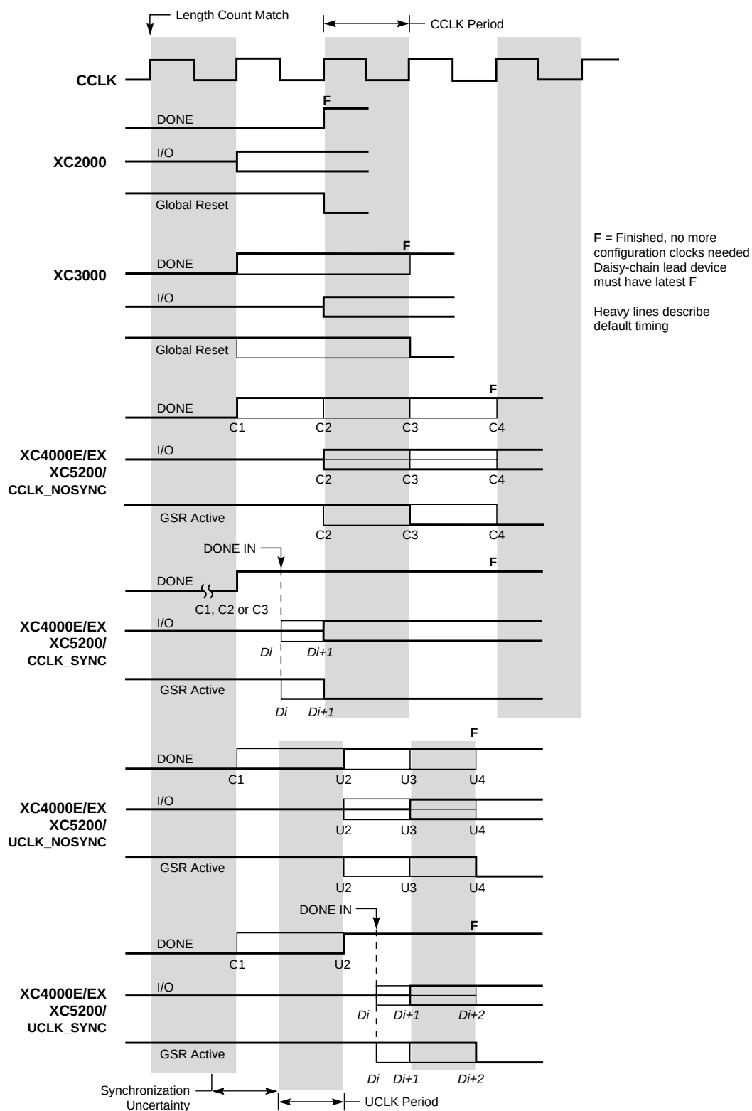
Figure 25: Start-up Timing
