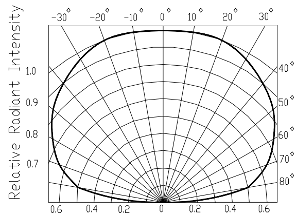
Fig. 6 Relative Radiant Intensity Angular Displacement
