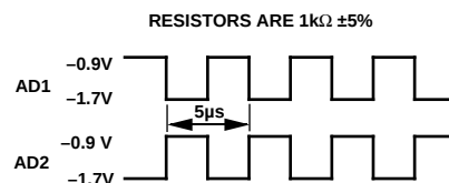
Burn-In Circuit
