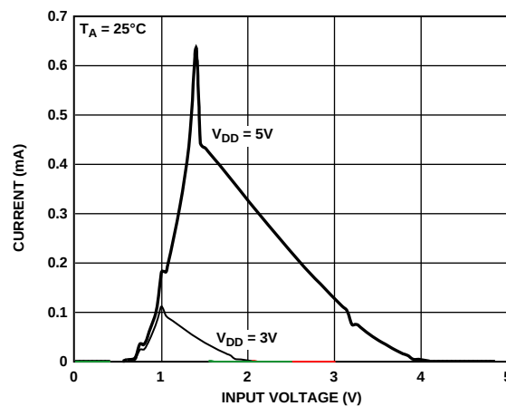
Figure 21. Supply Current vs. Logic Input Voltage, \overline{\text{SYNC}} (SCLK), DATA = 0
